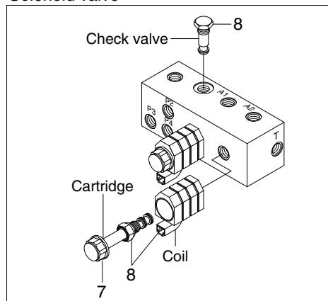
Solenoid valve
